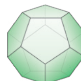
Dodecaedru regulat
