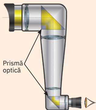
Periscop
