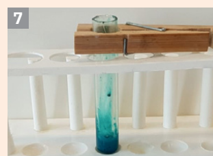
Hidroxid de cupru (II), \text{Cu(OH)}_2
