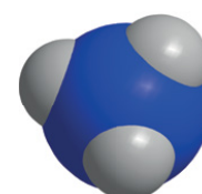
Amoniac
